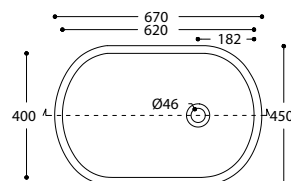
TOP VIEW * overflow
