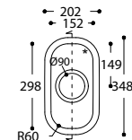
TOP VIEW * overflow
