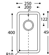
TOP VIEW * overflow
