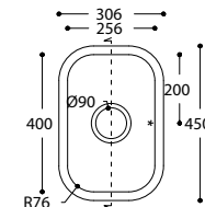
TOP VIEW * overflow
