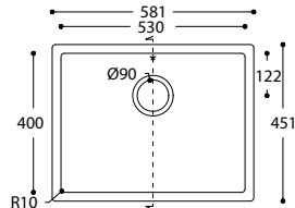
TOP VIEW * overflow
