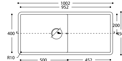
TOP VIEW * overflow
