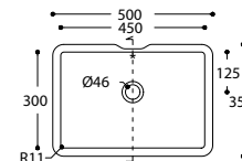
TOP VIEW * overflow
